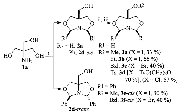
Scheme 3. i: 2 equiv. R 1 –CH=O, toluene, p TsOH, Dean–Stark, reflux; ii: 1.05 equiv. KH, THF, 40 °C, 1.5 h; iii: 1.05–1.10 equiv. R 2 X, THF, 40 °C to room temp., 12–24 h
