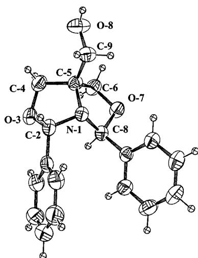
Figure 6. The X-ray crystallographically determined structure of compound 2d-trans and selected bond lengths [Å]: N-1–C-5 1.4935(17), N-1–C-2 1.4693(16), C-2–O-3 1.4287(16), O-3–C-4 1.4282(18), N-1–C-8 1.4855(16), C-8–O-7 1.4187(15), O-7–C-6 1.4329(16)
