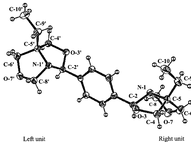
Figure 7. The X-ray crystallographically determined structure of compound 7c and selected bond lengths [Å]: N-1–C-5 1.493(4), N-1'–C-5' 1.498(3), N-1–C-2 1.479(3), N-1'–C-2' 1.467(3), C-2–O-3 1.407(3), C-2'–O-3' 1.419(3), O-3–C-4 1.436(3), O-3'–C-4' 1.433(3), N-1–C-8 1.454(4), N-1'–C-8' 1.449(3), C-8–O-7 1.426(4), C-8'–O-7' 1.428(3), O-7–C-6 1.409(4), O-7'–C-6' 1.428(3)
