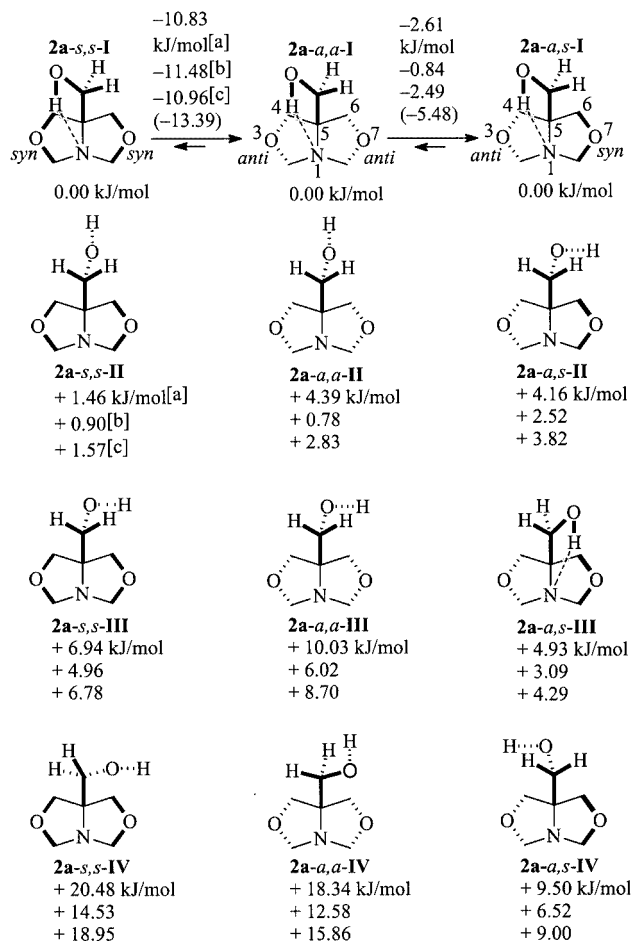
Scheme 6. [a] \Delta E values in vacuo and in the gas phase; [b] in DMSO; [c] in toluene; (in parentheses): \Delta E values obtained by neglecting the orientation of the hydroxymethyl group [21]
