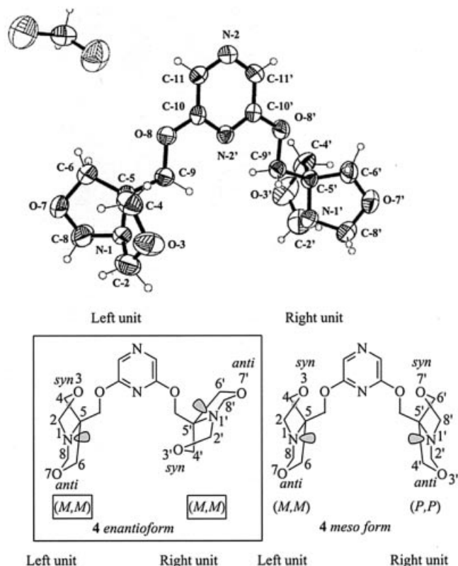
Figure 5. The X-ray crystallographically determined structure of compound 4 and selected bond lengths [Å]: chiral-4 : N-1–C-5 1.493(3), N-1'–C-5' 1.480(3), N-1–C-2 1.454(4), N-1'–C-2' 1.466(4), C-2–O-3 1.398(4), C-2'–O-3' 1.355(5), O-3–C-4 1.440(4), O-3'–C-4' 1.443(5), N-1–C-8 1.448(4), N-1'–C-8' 1.454(4), C-8–O-7 1.403(4), C-8'–O-7' 1.405(4), O-7–C-6 1.430(3), O-7'–C-6' 1.420(4); meso-4 : N-1–C-5 1.493(3), N-1'–C-5' 1.480(3), N-1–C-2 1.466(4), N-1'–C-2' 1.454(4), C-2–O-3 1.62(3), C-2'–O-3' 1.398(4), O-3–C-4 1.21(2), O-3'–C-4' 1.440(4), N-1–C-8 1.448(4), N-1'–C-8' 1.454(4), C-8–O-7 1.403(4), C-8'–O-7' 1.318(19), O-7–C-6 1.430(3), O-7'–C-6' 1.55(2)
