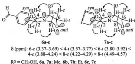
Scheme 10
