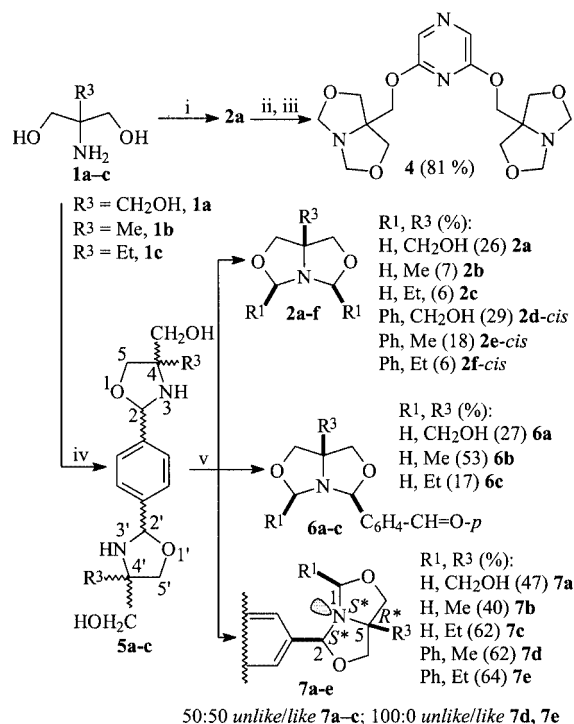
Scheme 4. i: R 3 = CH 2 OH, 2 equiv. CH 2 =O; [21] ii: 1.05 equiv. KH, THF, 40 °C, 1.5 h; iii: 0.48 equiv. 2,6-dichloropyrazine, THF, 60 °C to room temp., 24 h; iv: 0.5 equiv. terephthalaldehyde; [26] v: 2 equiv. R 1 –CH=O, toluene, p TsOH, Dean–Stark, reflux
