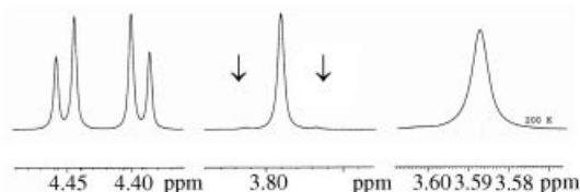
Figure 2. 1 H NMR spectra of compound 2a in [D 4 ]MeOD (400 MHz)
