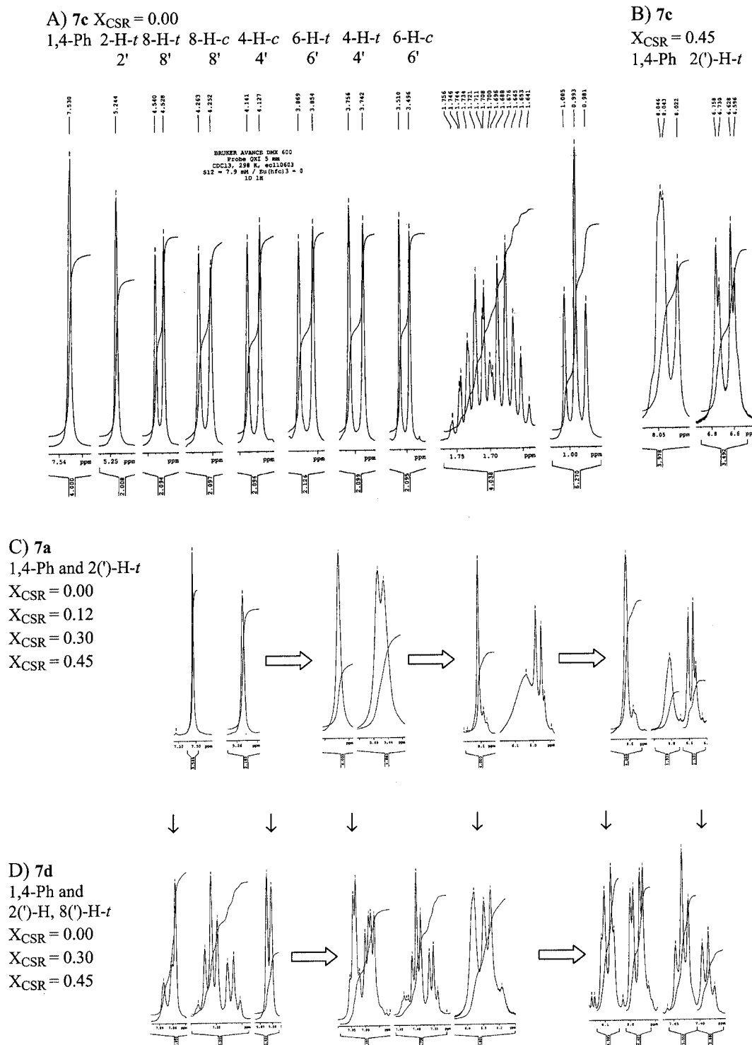
Figure 3. ^1\text{H} NMR spectra of compounds 7c (A, B), 7a (C, details) and 7d (D, details) before and after addition of increasing amounts of \text{Eu}(\text{hfc})_3 (see also Table 2)
