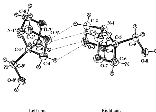
Figure 4. The X-ray crystallographically determined structure of compound 2a and selected bond lengths [Å]: N-1–C-5 1.499(3), N-1′–C-5′ 1.499(2), N-1–C-2 1.474(3), N-1′–C-2′ 1.467(3), C-2–O-3 1.420(3), C-2′–O-3′ 1.417(3), O-3–C-4 1.433(3), O-3′–C-4′ 1.416(3), N-1–C-8 1.466(3), N-1′–C-8′ 1.457(3), C-8–O-7 1.420(3), C-8′–O-7′ 1.415(3), O-7–C-6 1.420(3), O-7′–C-6′ 1.417(3).
