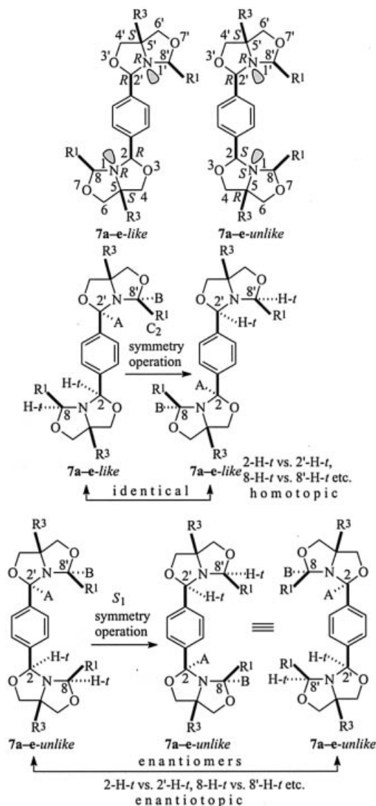
Scheme 11
