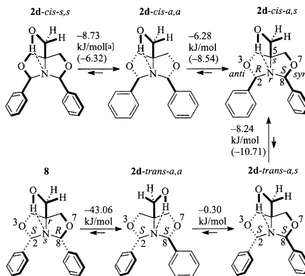
Scheme 7. [a] \Delta E values taking into account the orientation of the hydroxymethyl group; (in round parentheses): \Delta E values obtained by neglecting the orientation of the hydroxymethyl group [21]
