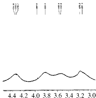
Figure 1. 1 H NMR spectrum of compound 2a in [D 8 ]toluene at the coalescence temperature (203 K, 400 MHz)
