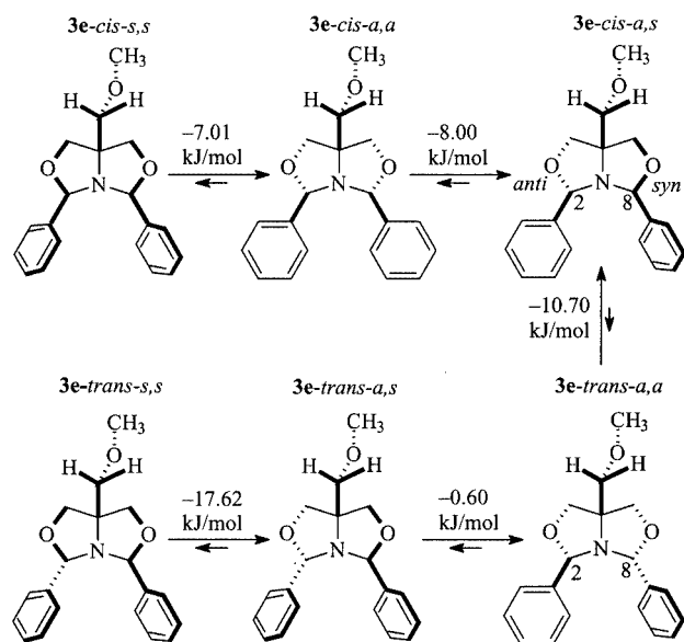
Scheme 9
